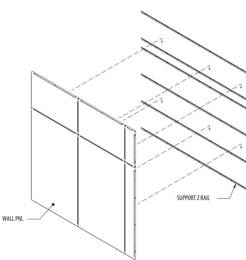
TYPICAL WALL PANEL SYSTEM
